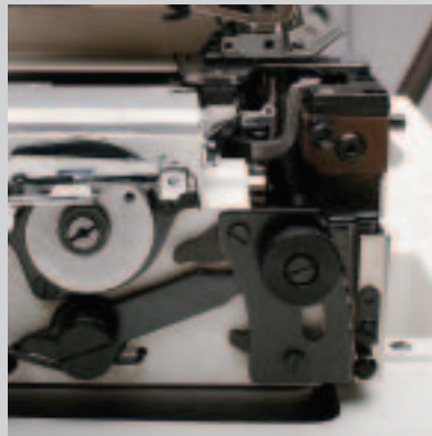
Differenzialtransportschnellverstellung Quick-change differential feed
